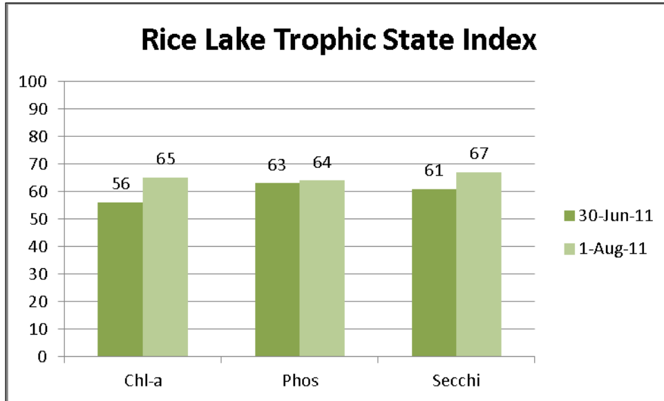
Figure 10: TSI
