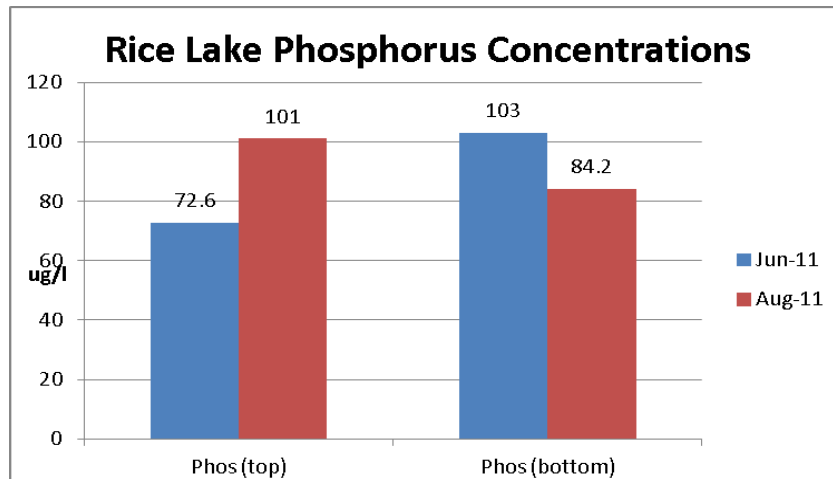
Figure 8: Total Phosphorus
